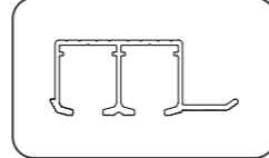
Upper rail(double door)
